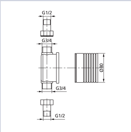
Concealed pipe interruptor, according to DIN 1988
