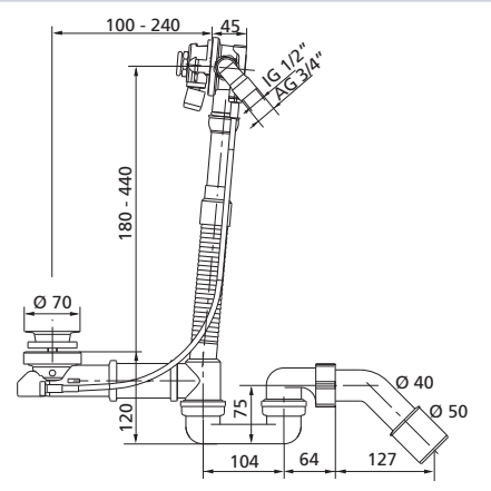
SANIT functional unit 836, for bath carrier
