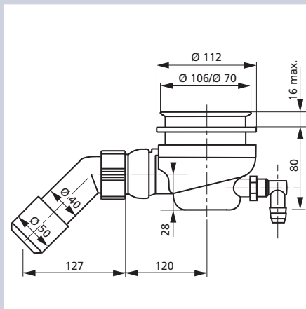
SANIT functional unit 821 with additional connector
